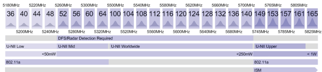
Figure 2: U-NII Frequency Spectrum
